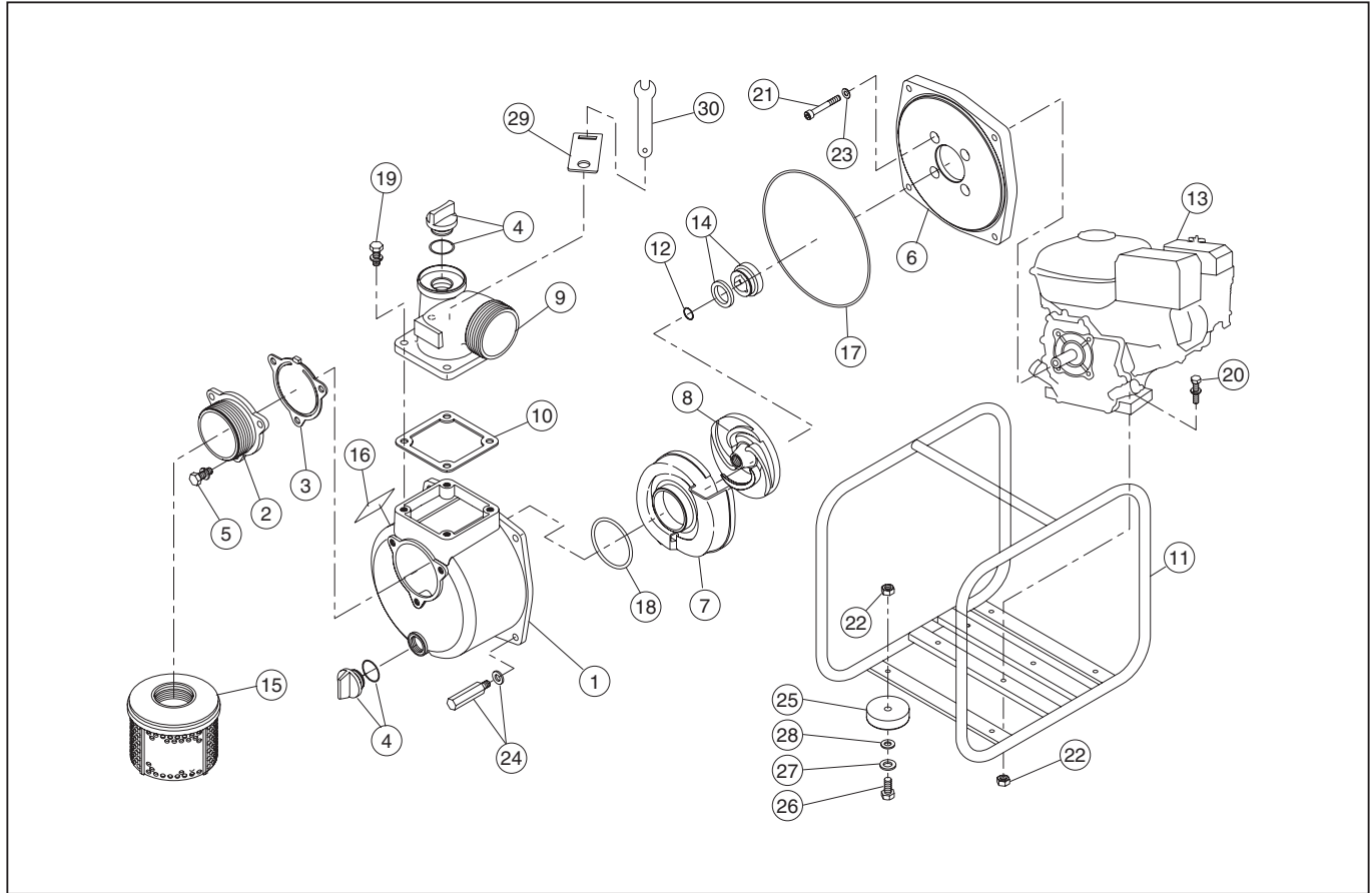
DWG NO.011980107 MODEL:SEH-50X FORM:SEH-50X-BCM
